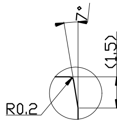
Detail K
